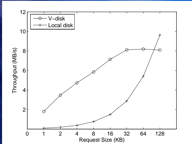
Read, unbuffered in Windows
