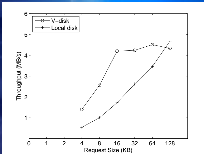
Read, unbuffered in Linux
